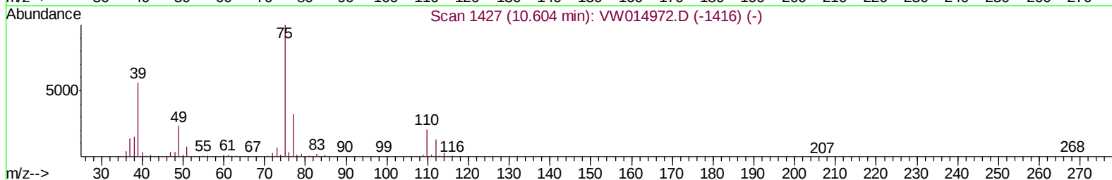
TIC: VW014982.D
