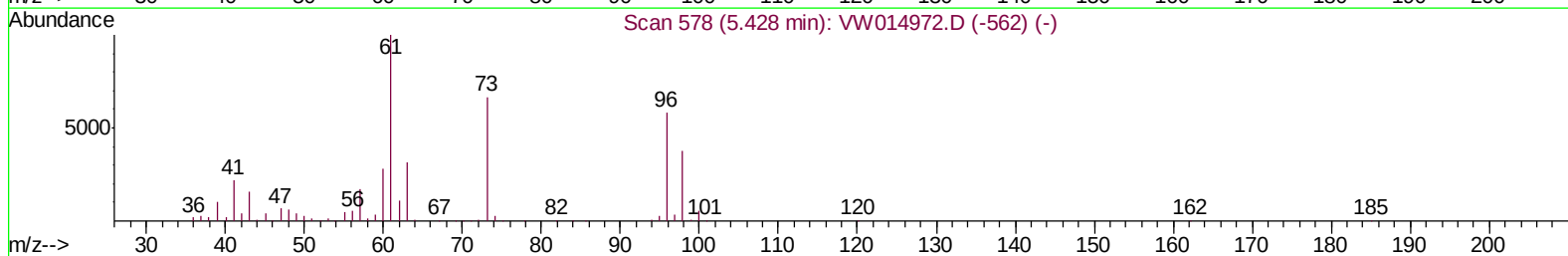
TIC: VW014981.D
