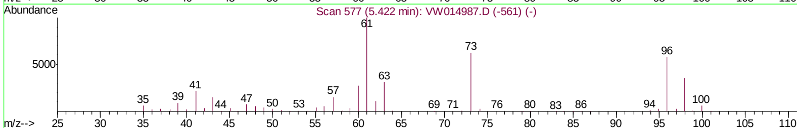
TIC: VW014991.D
