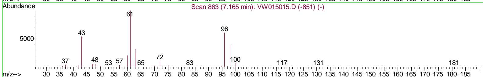
TIC: VW015017.D
