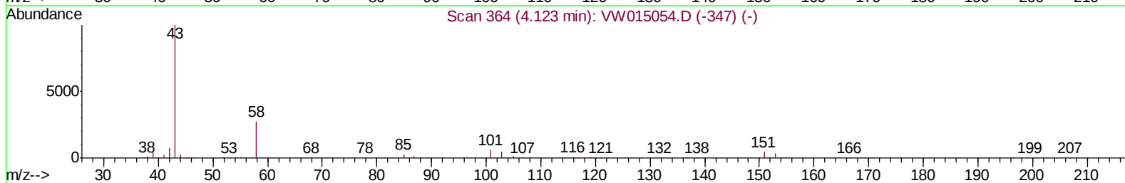
TIC: VW015063.D
