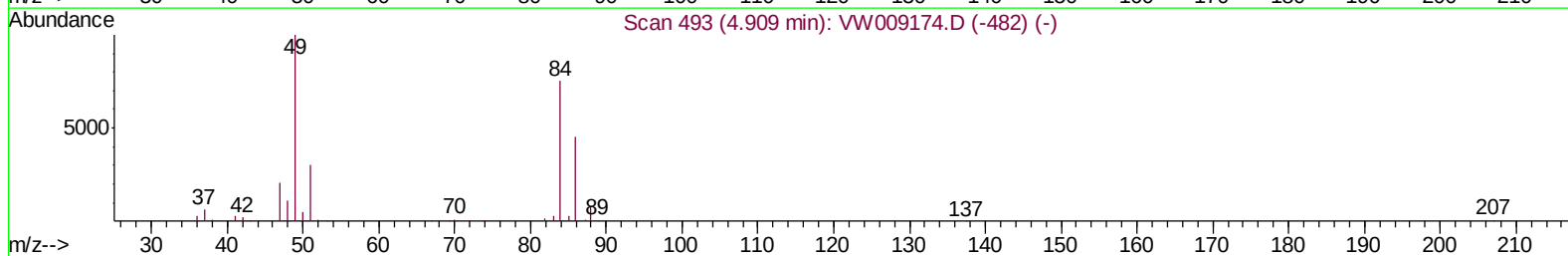
TIC: VW009189.D
