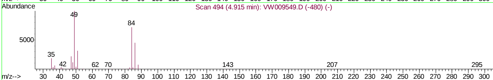
TIC: VW009553.D
