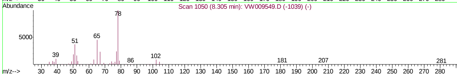
TIC: VW009555.D
