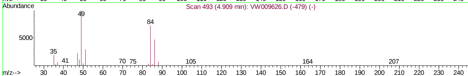
TIC: VW009632.D
