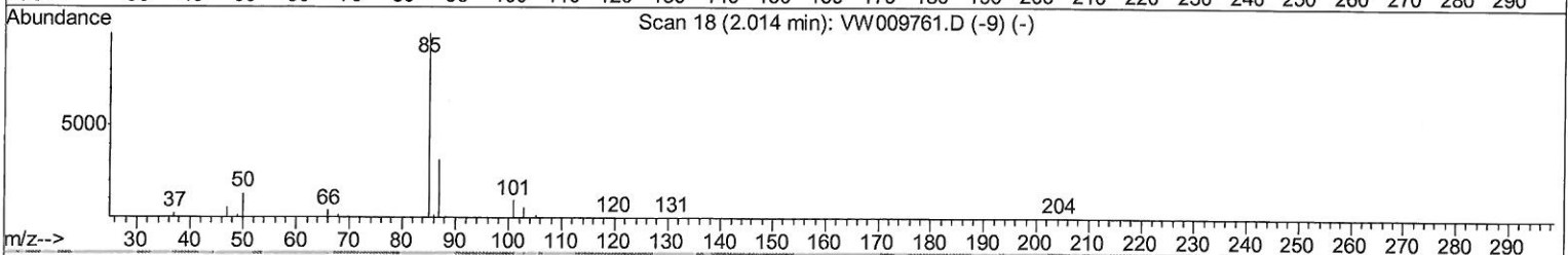
TIC: VW009781.D
