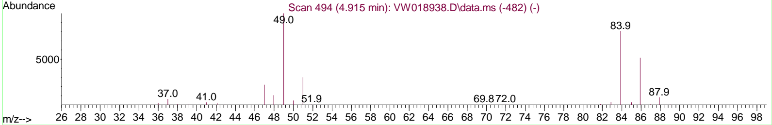
TIC: VW018940.D\data.ms
