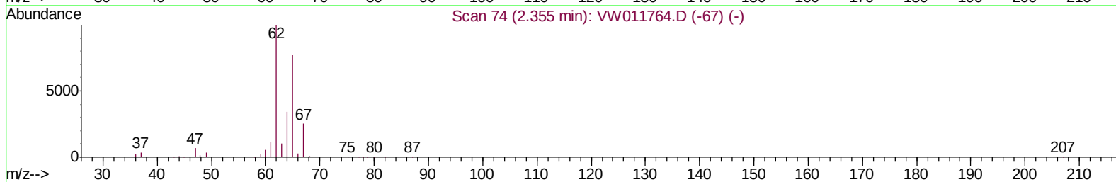
TIC: VW011769.D
