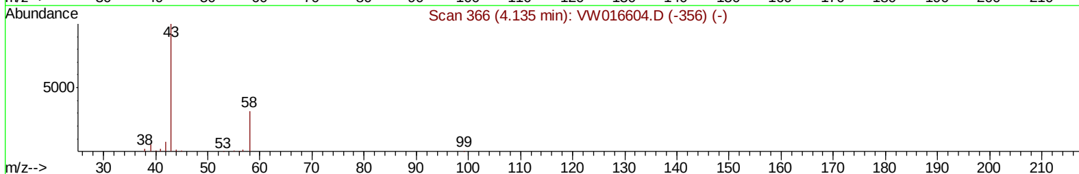
TIC: VW016610.D
