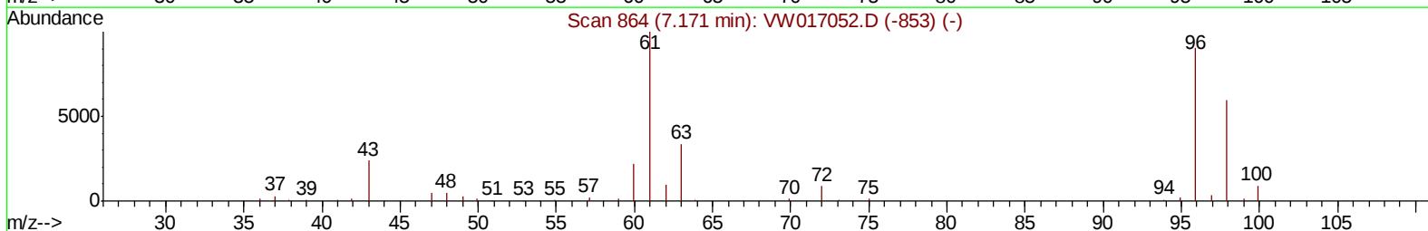
TIC: VW017056.D
