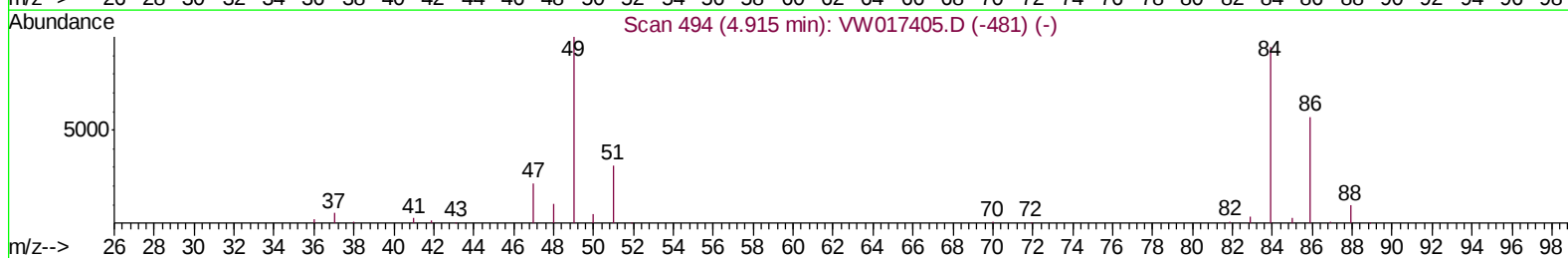
TIC: VW017423.D
