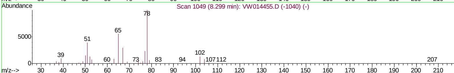
TIC: VW014460.D
