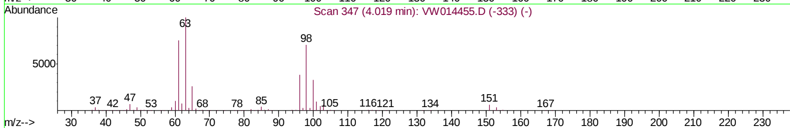
TIC: VW014464.D
