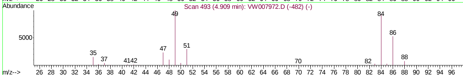
TIC: VW007975.D
