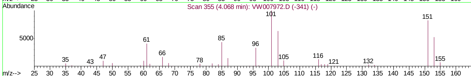
TIC: VW007992.D
