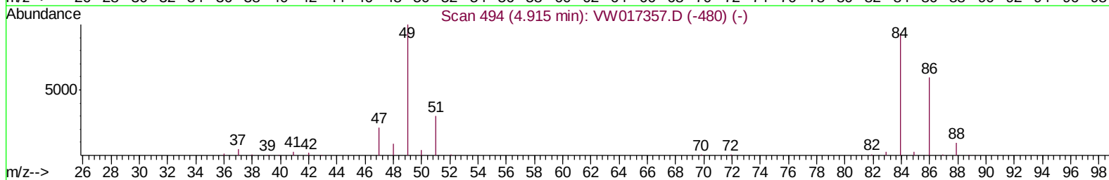
TIC: VW017376.D
