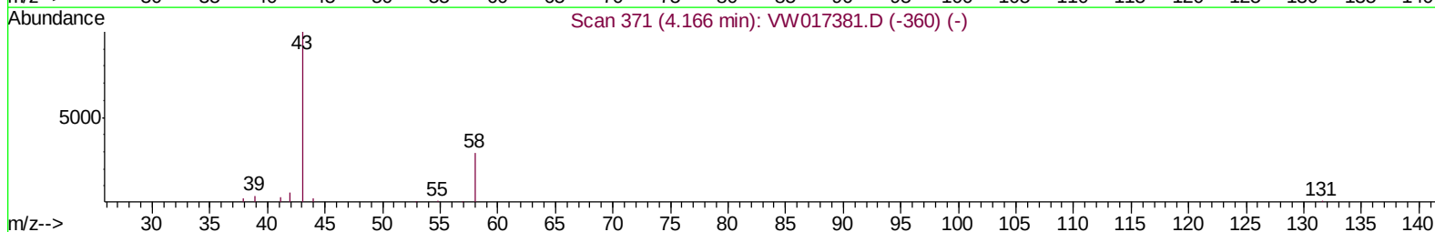
TIC: VW017394.D
