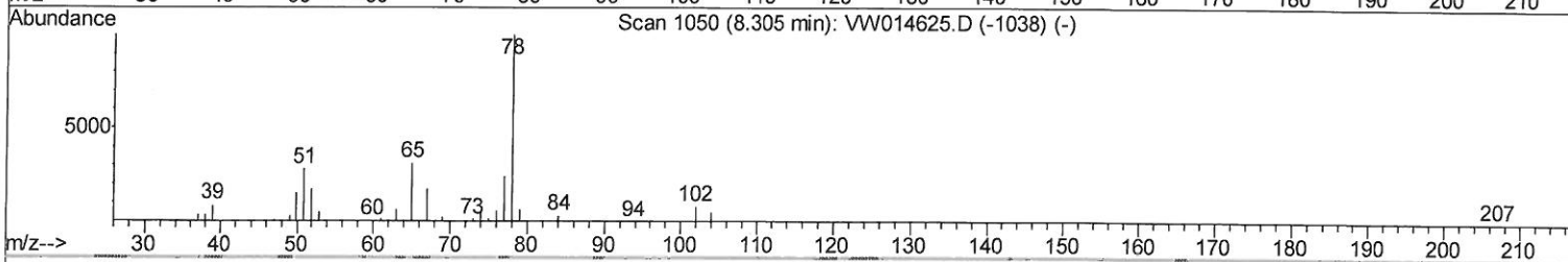
TIC: VW014626.D
