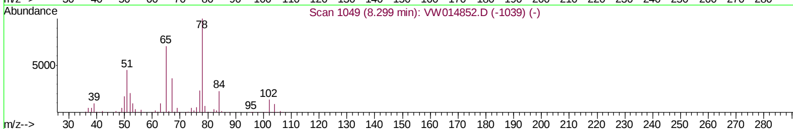
TIC: VW014861.D
