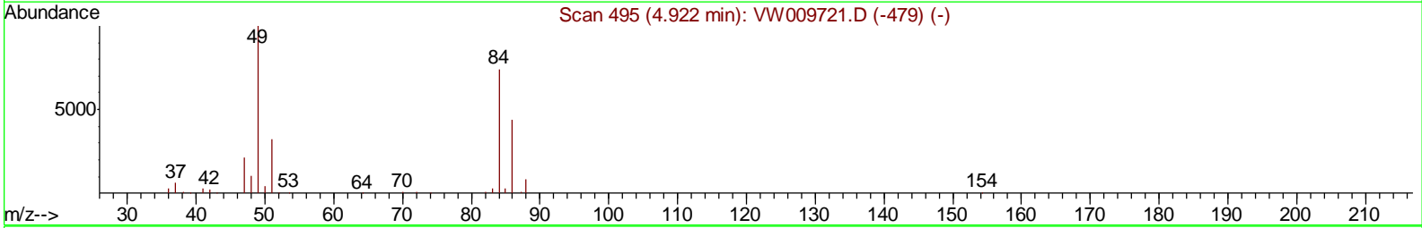
TIC: VW009733.D
