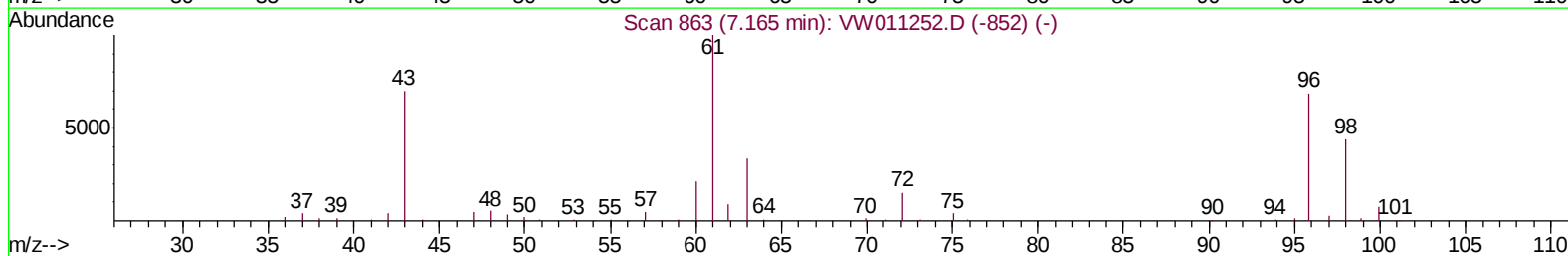
TIC: VW011270.D
