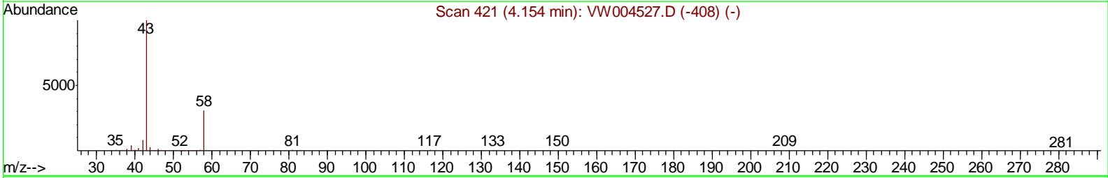
TIC: VW004528.D
