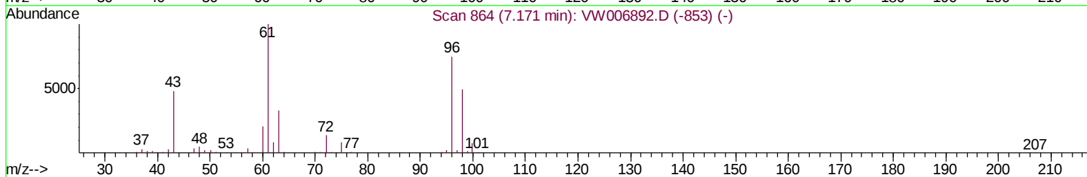
TIC: VW006894.D
