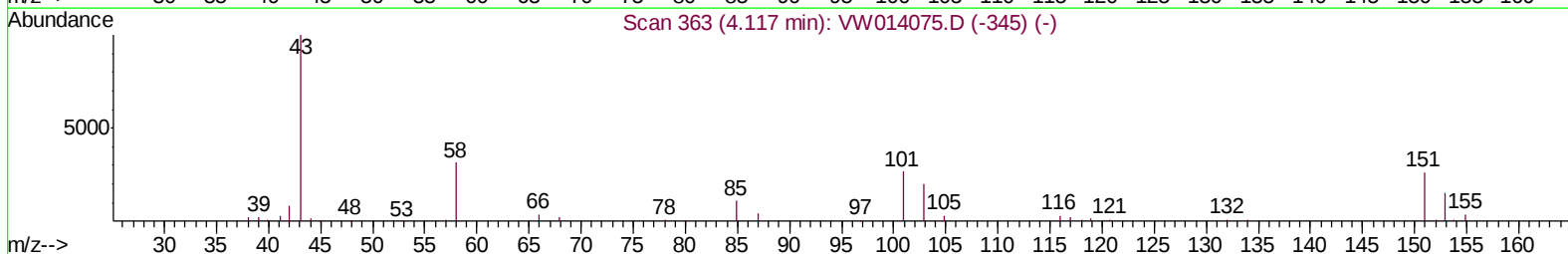
TIC: VW014078.D
