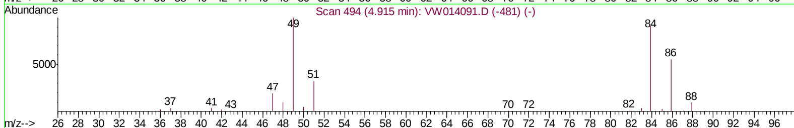
TIC: VW014093.D
